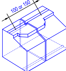
Cill Mullion stooled to C7 chamfered
